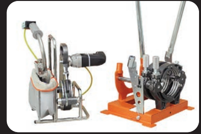
RITMO DELTA 160M BUTT FUSION MACHINE
